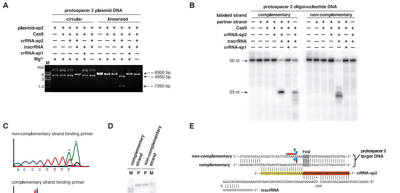
Fig. 1. Cas9 is a DNA endonuclease guided by two RNA molecules. (A) Cas9 was programmed with a 42-nucleotide crRNA-sp2 (crRNA containing a spacer 2 sequence) in the presence or absence of 75-nucleotide tracrRNA. The complex was added to circular or XhoI-linearized plasmid DNA bearing a sequence complementary to spacer 2 and a functional PAM. crRNA-sp1, specificity control; M, DNA marker; kbp, kilo-base pair. See fig. S3A. (B) Cas9 was programmed with crRNA-sp2 and tracrRNA (4). The complementary or noncomplementary strands of the DNA were 5'-radiolabeled and annealed with a nonlabeled partner strand. nt, nucleotides. See fig. S3, B and C. (C) Sequencing analysis of cleavage products from Fig. 1A. Termination of primer extension in the sequencing reaction indicates the position of the cleavage site. The 3' terminal A overhang (asterisks) is an artifact of the sequencing reaction. See fig. S5, A and C. (D) The cleavage products from Fig. 1B were analyzed alongside 5' end-labeled size markers derived from the complementary and noncomplementary strands of the target DNA duplex. M, marker; P, cleavage product. See fig. S5, B and C. (E) Schematic representation of tracrRNA, crRNA-sp2, and protospacer 2 DNA sequences. Regions of crRNA complementarity to tracrRNA (orange) and the protospacer DNA (yellow) are represented. The PAM sequence is shown in gray; cleavage sites mapped in (C) and (D) are represented by blue arrows (C), a red arrow [(D), complementary strand], and a red line [(D), non-complementary strand].
